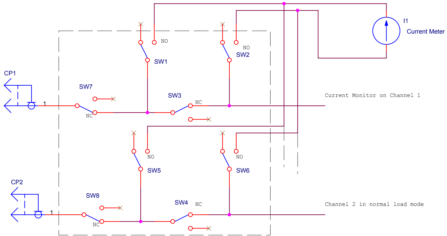
Two of 8ea HV Channels Illustrated
