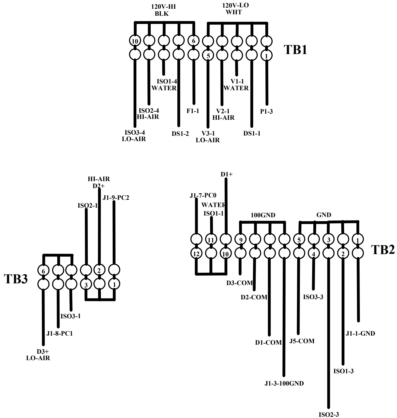
UCSB COLD BOX FLOW CONTROL WIRING
