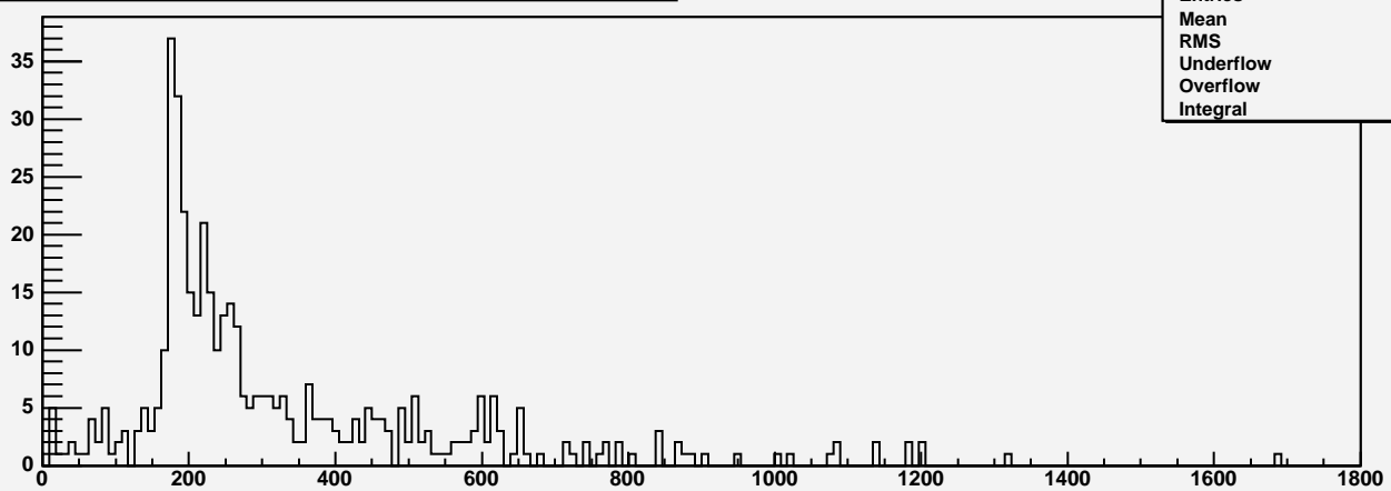
Invariant mass of Higgs from gammas, reconstruction level
