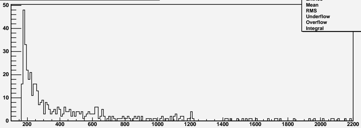
Invariant mass of Higgs from gammas, generator level
