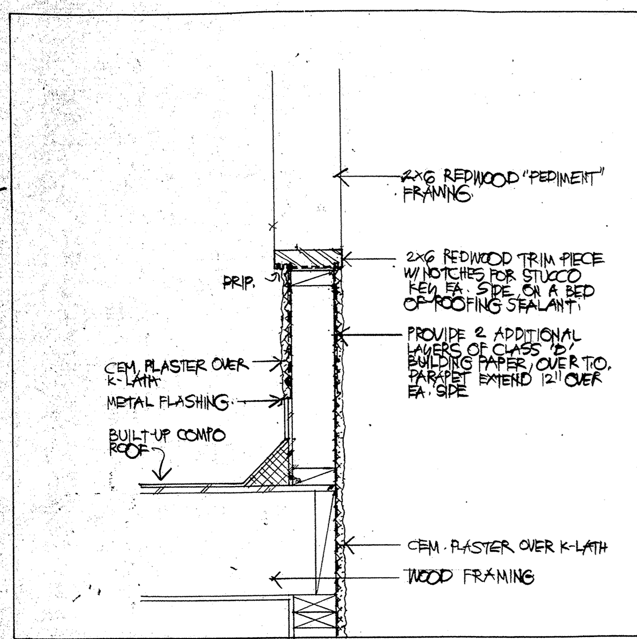
WOOD PEDIMENT 1/2"=1'-0"
