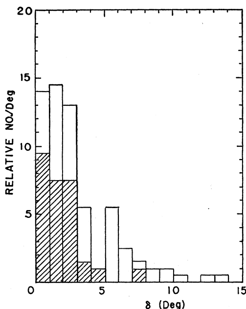
FIG. 8. Distribution of angular deviation \delta from coplanarity for 60 cases. The cross-hatched portion of the distribution represents the contribution of the 28 cases whose estimated errors of measurement were 2^\circ or less.
