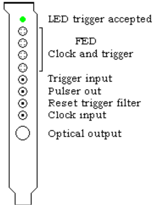
Figure 4. Front panel connectors
