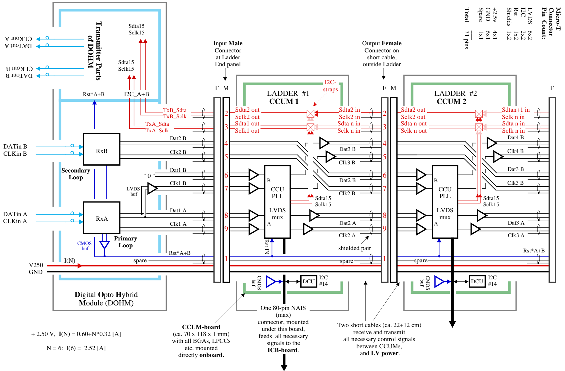
TOB CCUM Block Diagram for DS-layer 1-6 Control Signals
