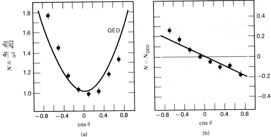
Fig. 13.7 (a) The \cos \theta distribution for the process e^- e^+ \rightarrow \mu^- \mu^+ does not follow the 1 + \cos^2 \theta QED prediction. (b) The discrepancy is explained by the interference of the virtual Z and \gamma contributions. (Compilation by R. Marshall.)
