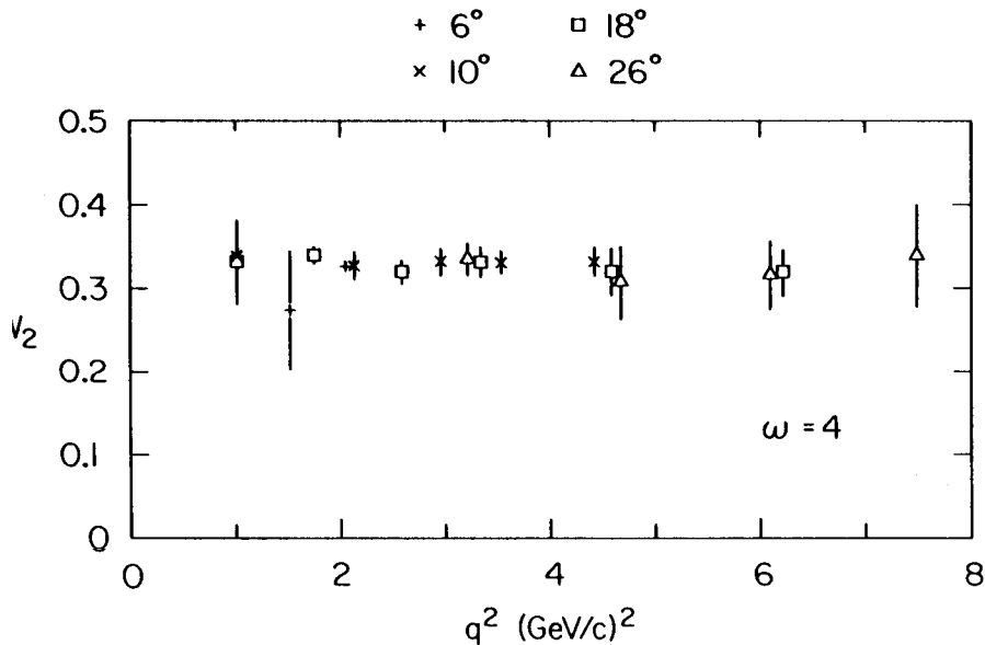
Fig. 13. An early observation of scaling: \bar{\nu}W_2^+ for the proton as a function of \hat{q}^2 for W > 2 GeV, at \omega = 4 .
