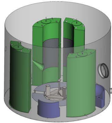
U3 - VESSEL SUPPORT LEGS
