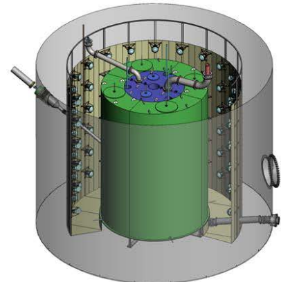
U9 - WATER PMTs
