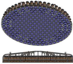
S1 - PMT ARRAYS - UPPER & LOWER
